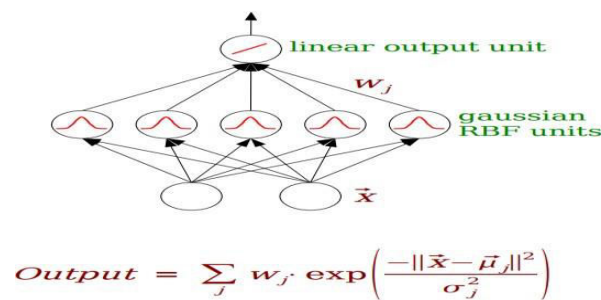
Fig -2: RBF Network
