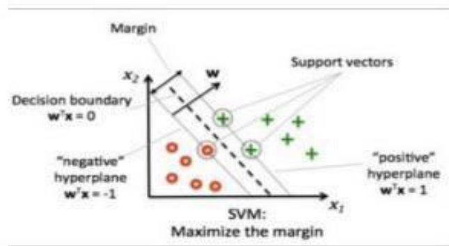
Fig -1: The Support Vector Machine Decision Making Boundary
