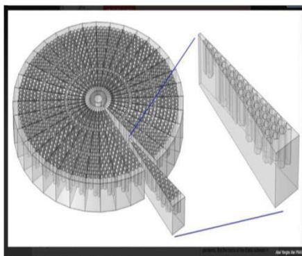
Fig 1: Shock Absorber
