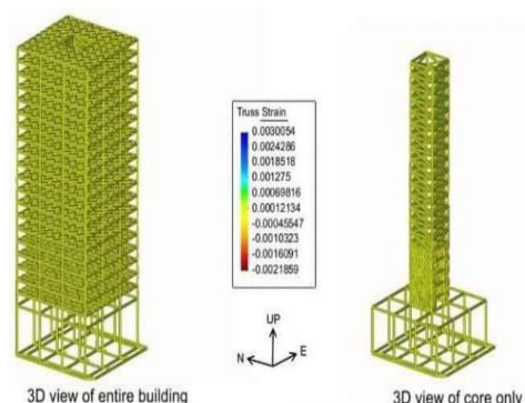
Fig 2: Rocking Core-Wall
