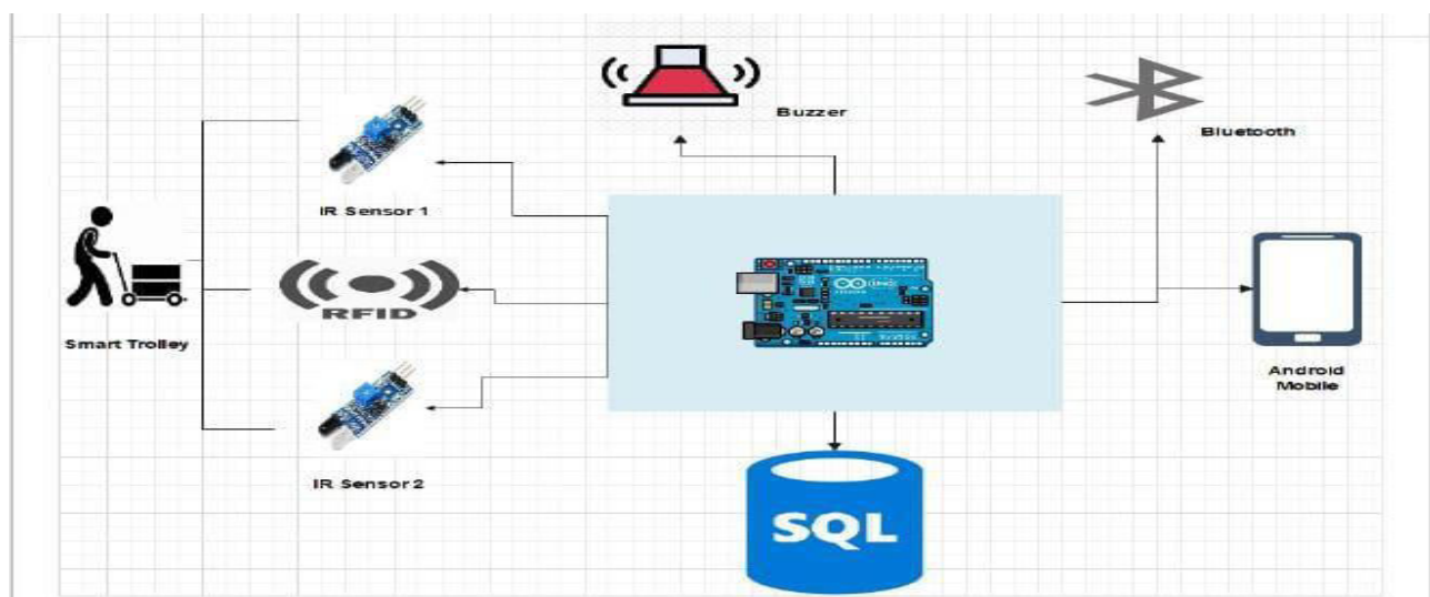
Fig 1. System Architecture
