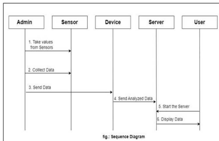
FIG 4.2: SEQUENNCE DIAGRAM
