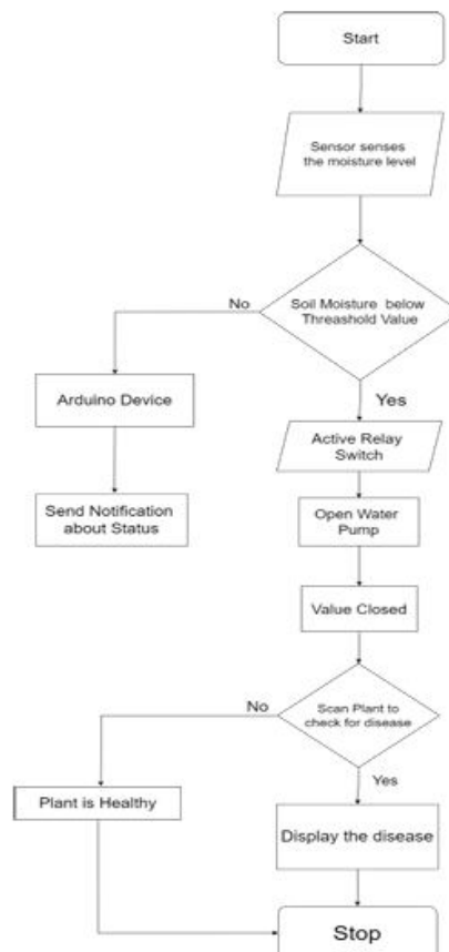
Fig 4.1: Flowchart of the application
