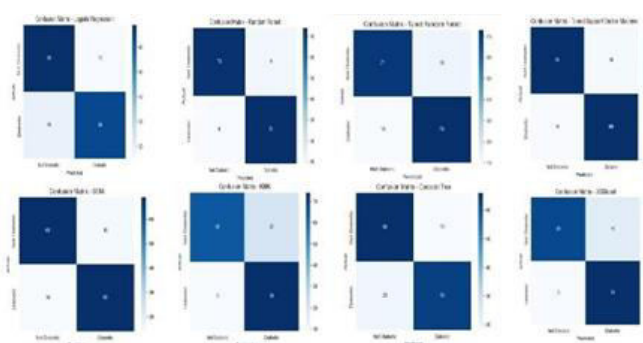
Fig. 5. Confusion Matrix
