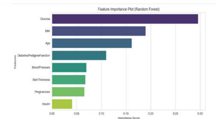
Fig. 3. Feature Importance Graph
