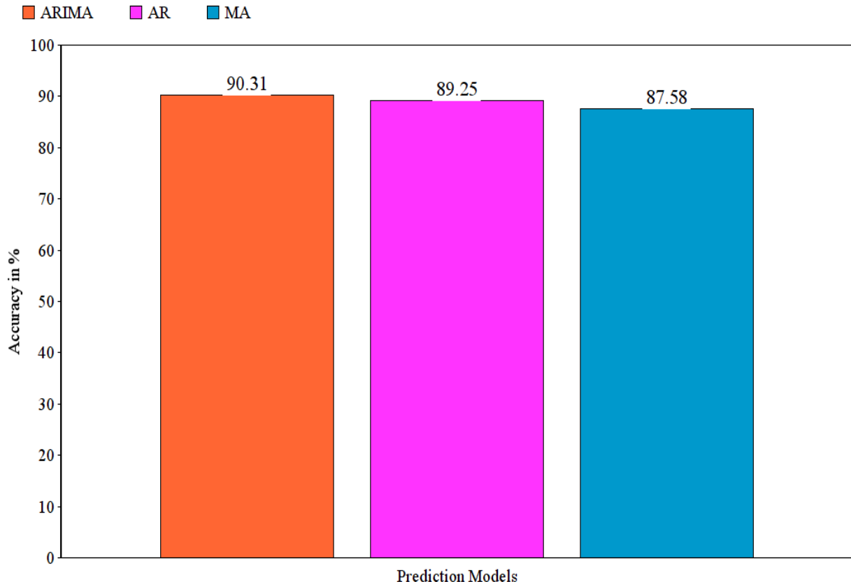
Fig. 8. Comparison barcharts between prediction Time Series Algorithms
