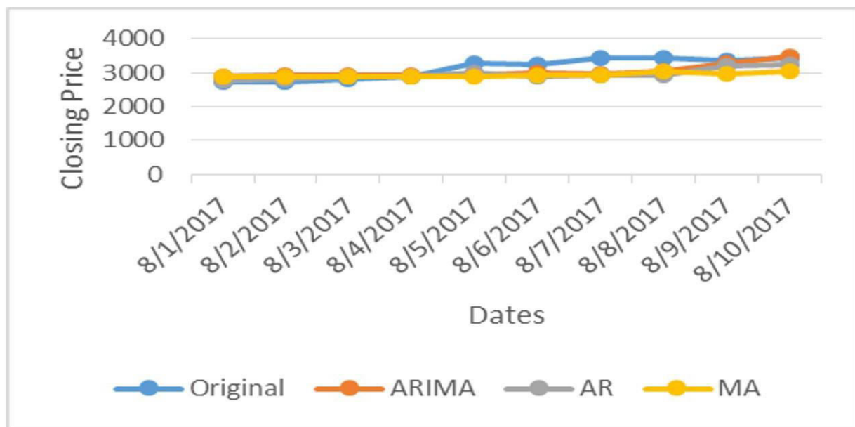
Fig. 7. Original Bitcoin price vs predicted bitcoin price of ARIMA, AR and MA
