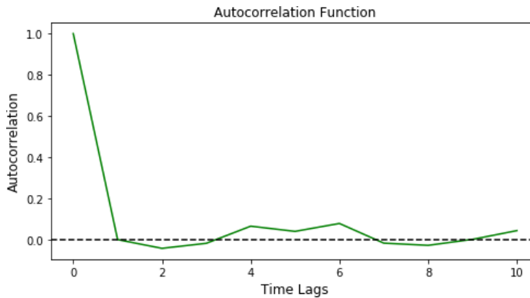
Fig. 3. Autocorrelation
