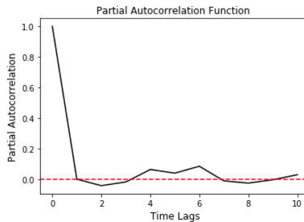
Fig. 4. Partial Autocorrelation
