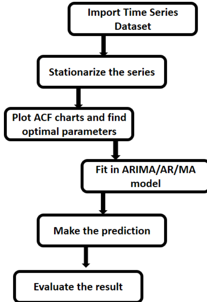
Fig. 5. Proposed Model of Time Series Analysis
