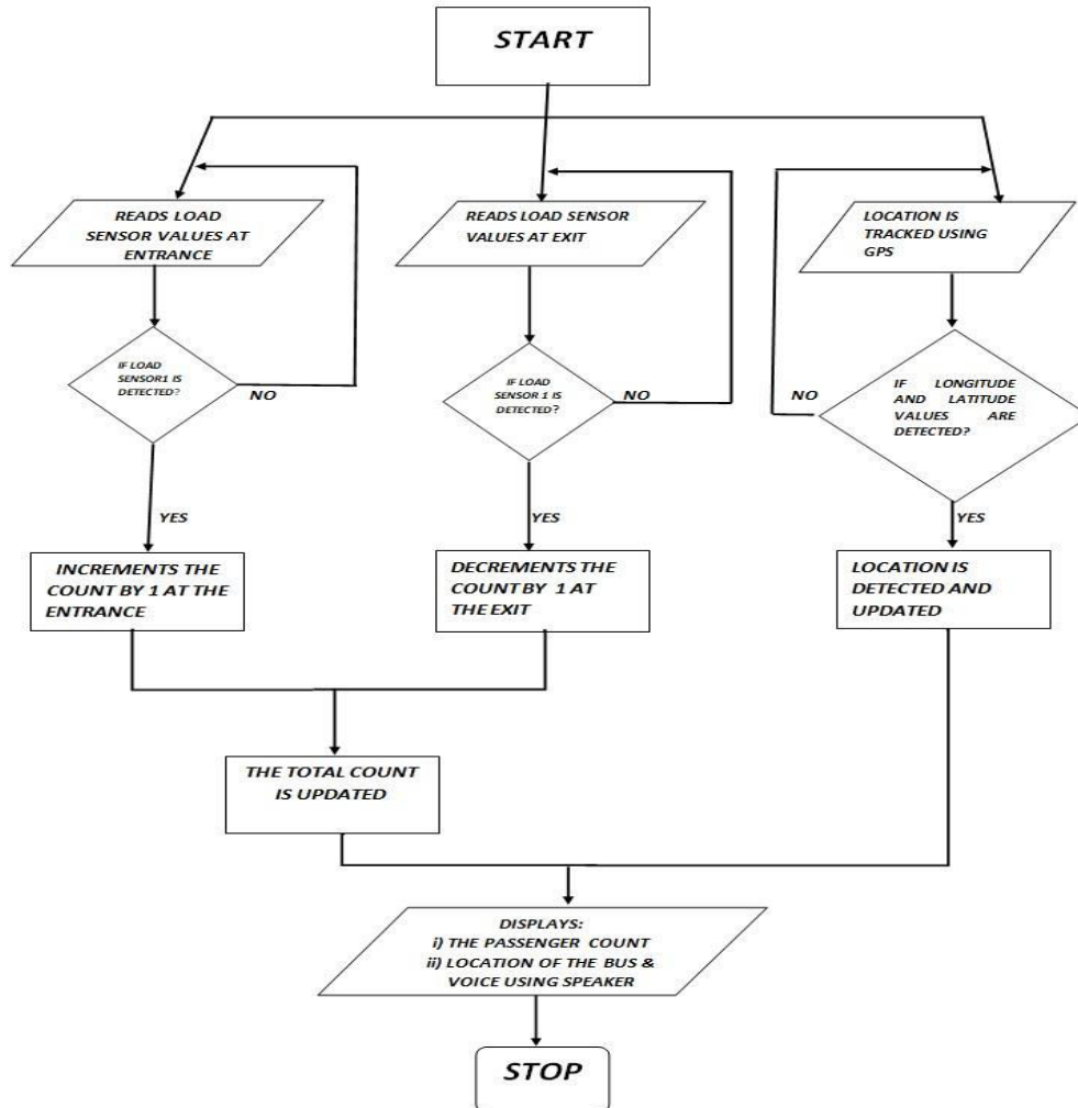
Fig.1: Flowchart for Real-Time Seat Availability System
