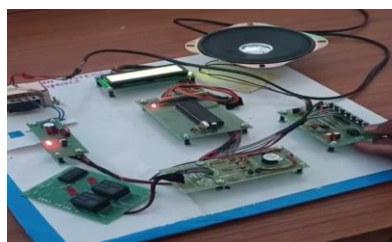
Fig.5: IoT-Driven Real-Time Seat Availability System
