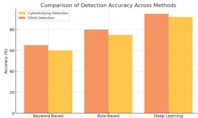
Figure 2: Comparison of Cyberbullying and DDoS Attack Detection Accuracy Across Methods
