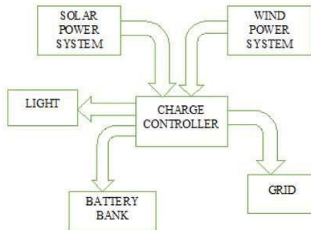
Figure3.1BlockDiagramofHybridPower Generation
