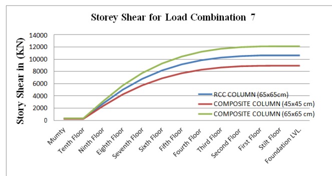
Chart -4: Storey Shear for Load Combination -7
