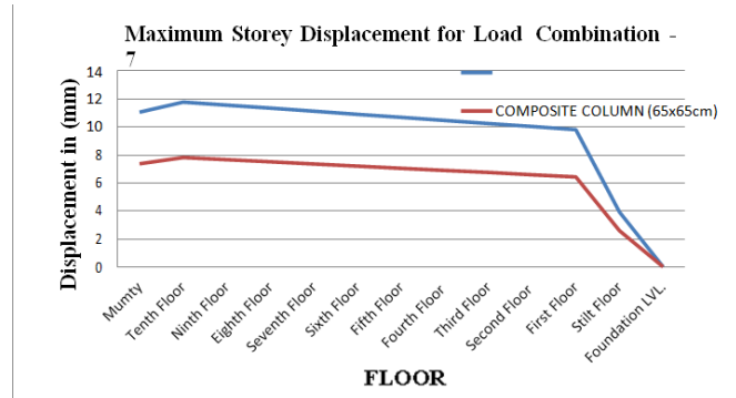
Chart -2: Maximum Storey Displacement for Load Combination -7
