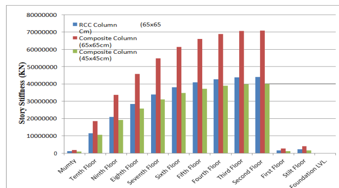
Chart -5: The Storey stiffness for models
