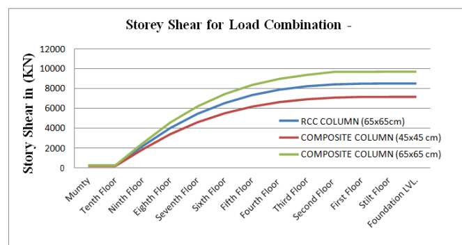
Chart -3: Storey Shear for Load Combination -2
