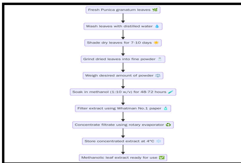
Figure 6: Flow diagram showing the extraction procedure for obtaining methanolic leaf extract of Punica granatum .
