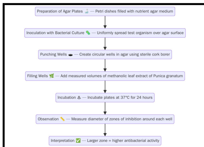
Figure 7: Schematic representation of the agar well diffusion assay used to evaluate antibacterial activity of methanolic leaf extract of Punica granatum .
