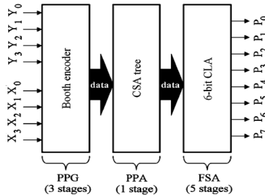
Fig.2 The Structure of Existing 4-Bit Parallel Multiplier.
