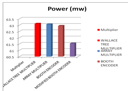
Figure 7 Power Analysis of Multipliers
