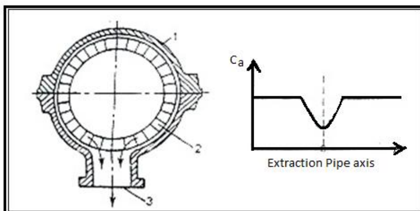
Fig.5: Formation of flow at an extraction pipe 1-Tubing casing , 2- Nozzle Cascade, 3-Steam extraction pipe
