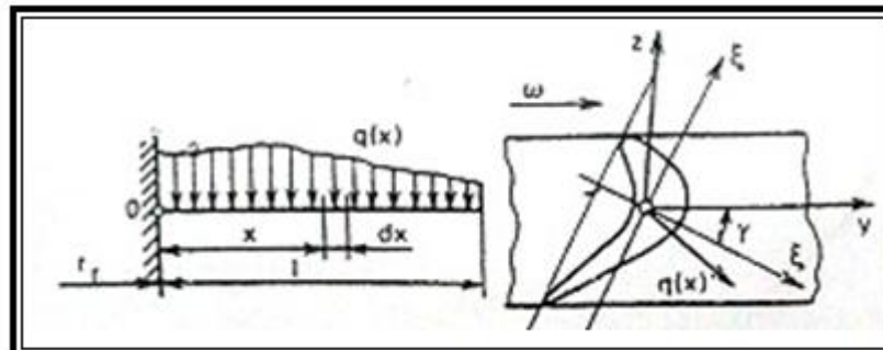
Fig.2: Diagram of blade stressing by bending forces.
