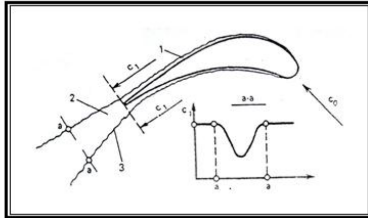
Fig.3: Formation of trailing trace behind a blade 1-Boundary on blade surface, 2-Trailing trace, 3-Boundary of trailing trace, C_0 -Incoming flow velocity, C_1 - Velocity of flow behind the blade
