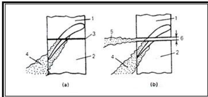
Fig.4: Formation of flow at the horizontal joint of a poorly manufactured diaphragm 1- Upper half diaphragm, 2- Lower half diaphragm, 3-Parting plane, 4-Verte tracing formed by Protrusions on nozzle blade, 5-Jet of working fluid flowing from the gap between diaphragm halves, 6- Gap between diaphragm halves
