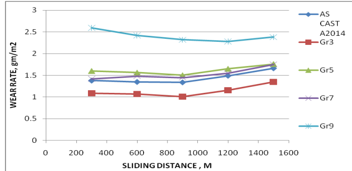
Fig 3.9: Wear rate of A2014 and its alloys
